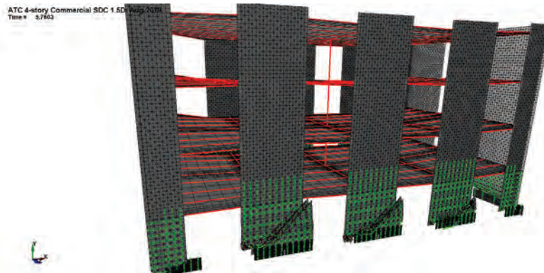
Figure B-59 Deformed meshes from refined model: COM6 (LS-DYNA) – Motion 2 ( 2 \times MCE_R ).
