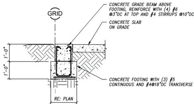
Figure A-30 Commercial building foundation detail at grade beam.
