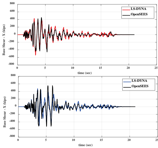
Figure B-21 Comparison of base-shear histories: COM2 – Motion 2 ( MCE_R ).
