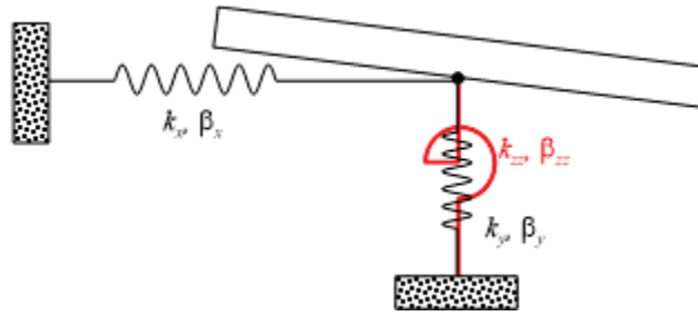
Figure C-2 Translational and rotational springs and dampers.
