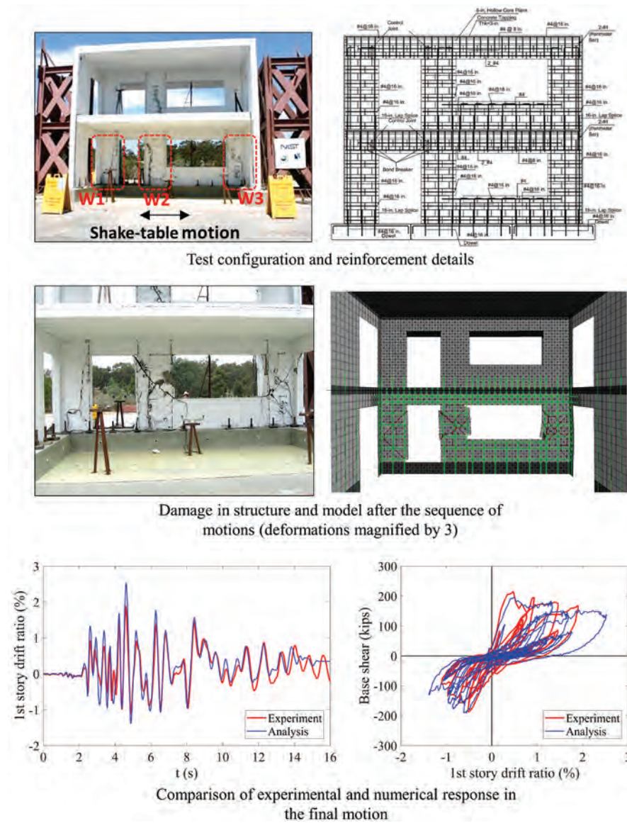
Figure 4-18 Two-story reinforced masonry wall structure tested by Mavros et al. (2016).
