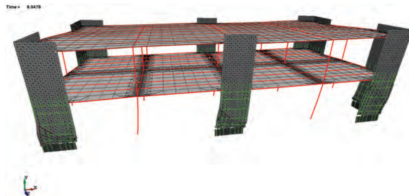
Figure B-46 Deformed meshes from refined model: COM5 (LS-DYNA) – Motion 2 ( 1.9 \times MCE_R ).
