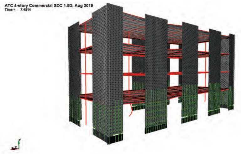
Figure B-60 Deformed meshes from refined model: COM6 (LS-DYNA) – Motion 17 ( 2 \times MCE_R ).
