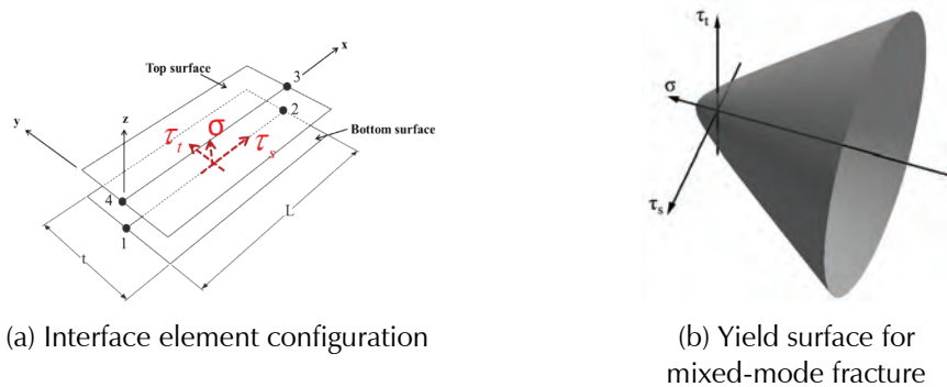
Figure 4-8 Cohesive-crack interface element.
