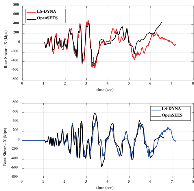
Figure B-22 Comparison of base-shear histories: COM2 – Motion 2 ( 2 \times MCE_R ).
