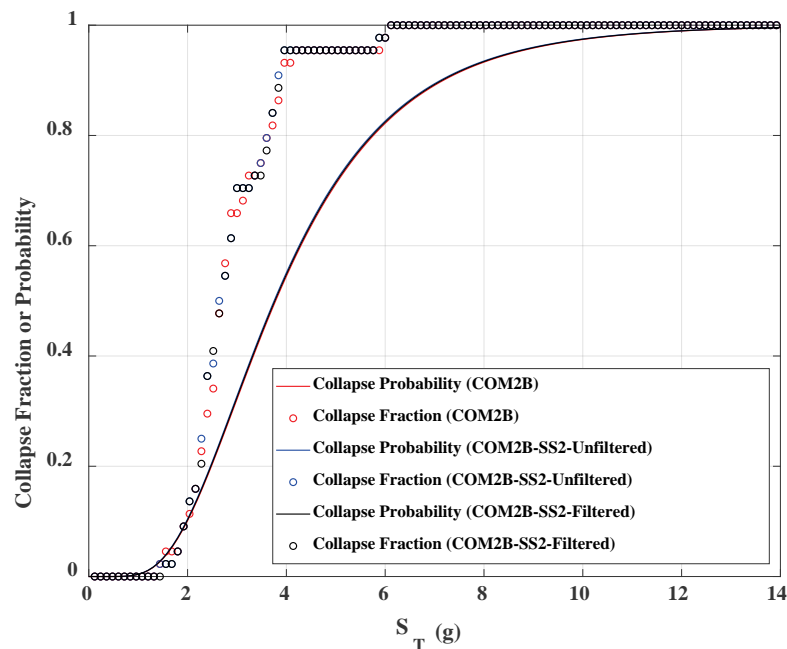
Figure 5-18 Collapse rates from IDA data and collapse fragility curves derived for COM2B and COM2B-SS2. S_T for the collapse fraction data has been scaled by 1.2, whereas that for the collapse probability curve has been scaled by 1.2 \times SSF .
