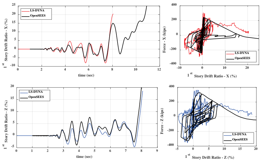
Figure B-5 Comparison of response histories for the first story: COM1 – Motion 1 ( 3.0 \times MCE_R ).
