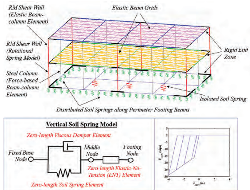
Modeling Scheme and Force-Displacement Relation for Vertical Soil Springs
