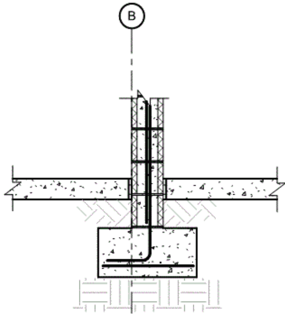
Figure A-46 Residential building foundation detail.
