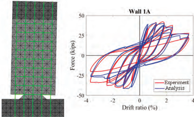
Figure 4-15 Flexure-dominated wall tested by Sherman (2011).
