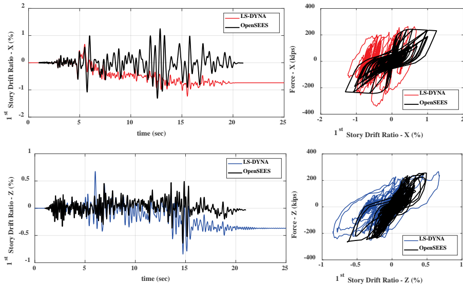
Figure B-8 Comparison of response histories for the first story: COM1 – Motion 17 ( 1.5 \times MCE_R ).
