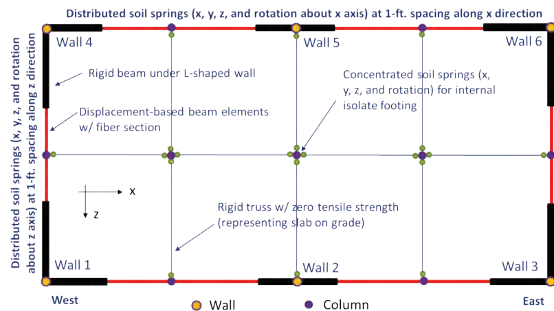
Figure 4-34 Foundation model for the soft site for SSI analyses.
