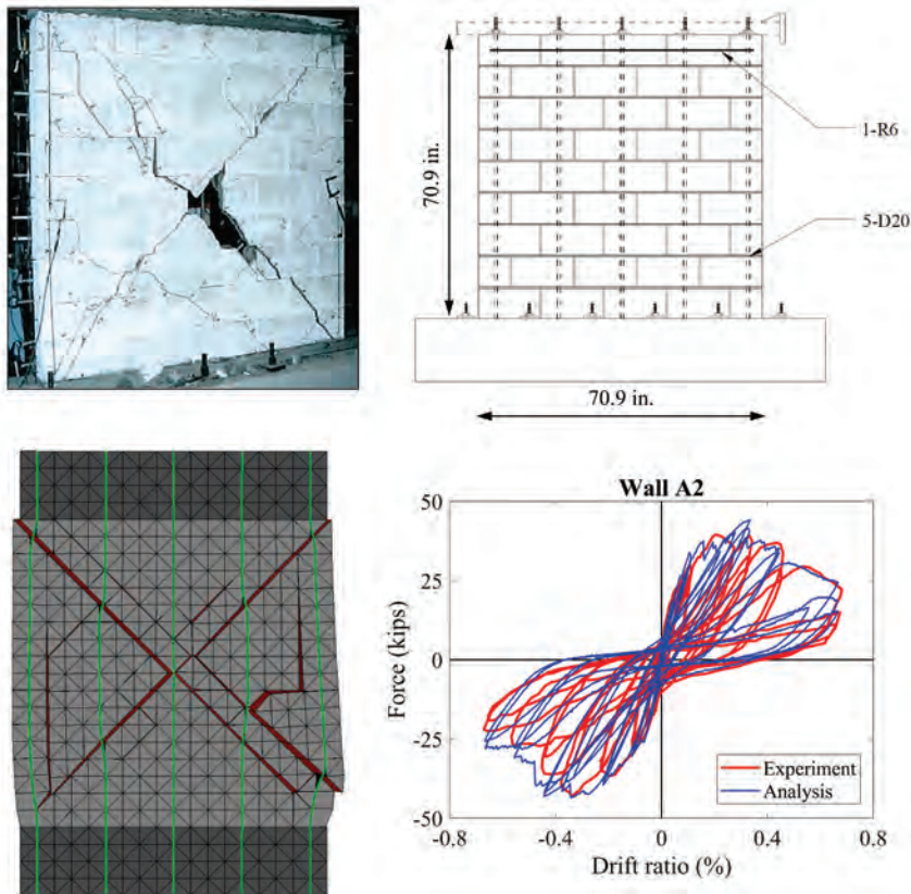
Figure 4-16 Shear-dominated wall tested by Voon and Ingham (2006).
