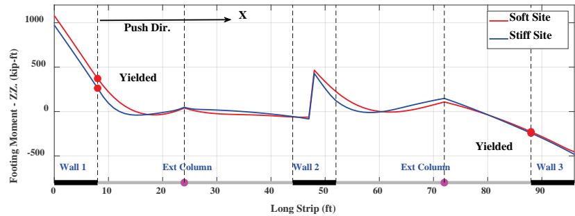
Figure 5-15 Moments in foundation slabs and grade beams for the stiff and soft sites at the respective maximum base shear.
