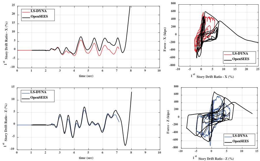
Figure B-49 Comparison of response histories for the first story: COM5 – Motion 1 ( 2 \times MCE_R ).
