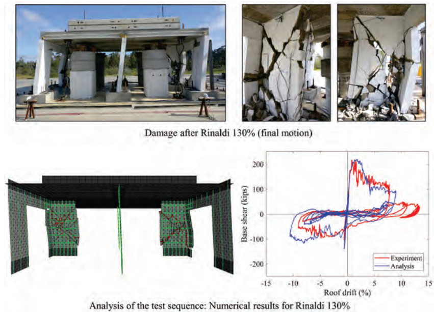
Figure 4-19 Reinforced masonry wall system tested to near collapse on a shake table (Cheng et al., 2020).
