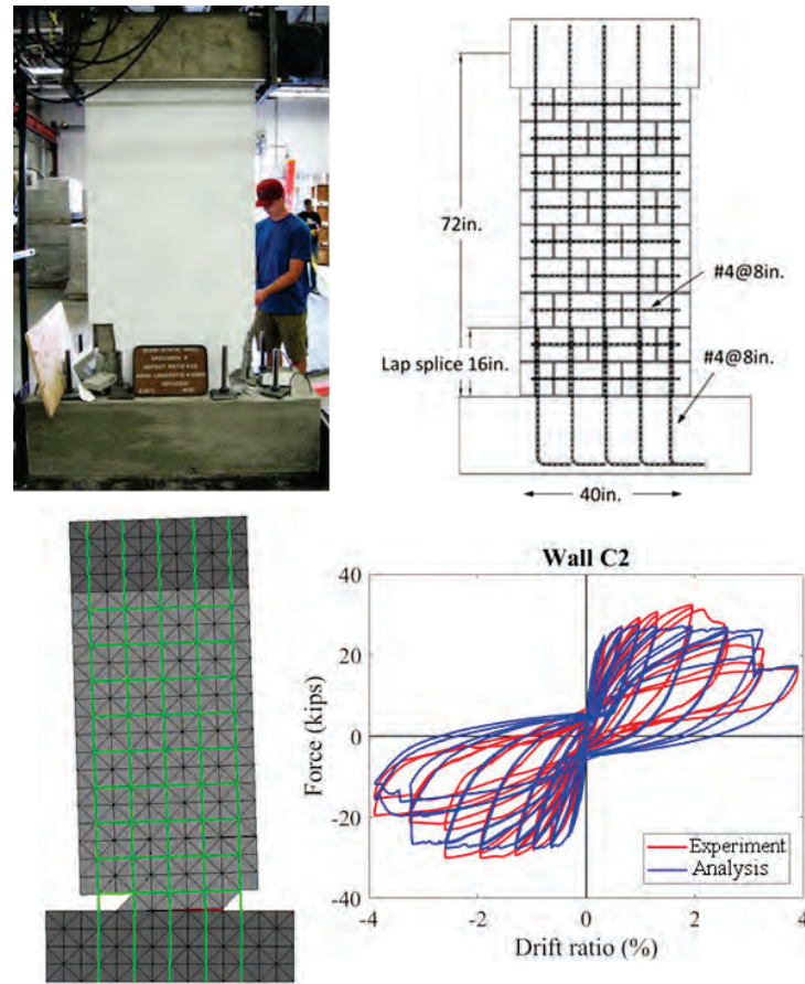
Figure 4-14 Flexure-dominated wall tested by Kapoi (2012).
