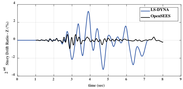
Figure B-55 Comparison of story-drift histories for the second story: COM5 – Motion 1 (2×MCE R ).
