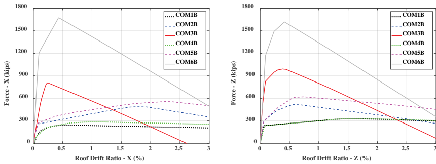
Figure 5-3 Zoomed-in pushover curves for all archetypes.
