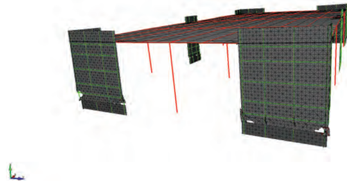
Figure B-3 Deformed meshes from refined model: COM1 (LS-DYNA) – Motion 17 ( 3 \times MCE_R ).
