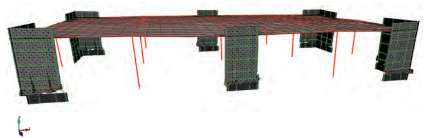
Figure B-2 Deformed meshes from refined model: COM1 (LS-DYNA) – Motion 2 ( 2.7 \times MCE_R ).
