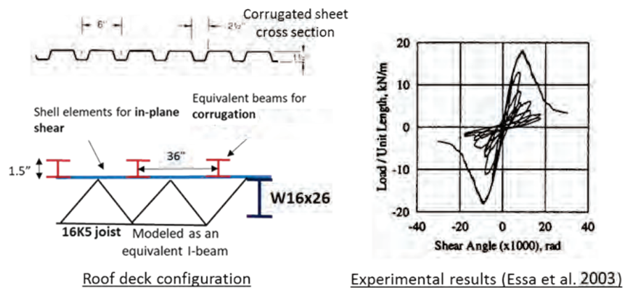
Figure 4-22 Modeling of roof diaphragm.
