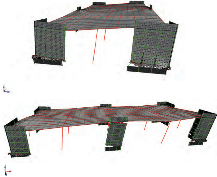
Figure B-1 Deformed meshes from refined model: COM1 (LS-DYNA) – Motion 1 ( 3 \times MCE_R ).
