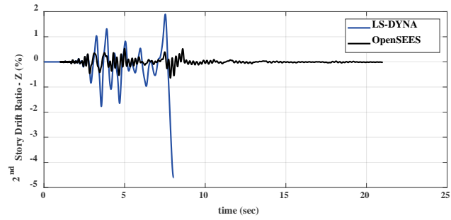
Figure B-54 Comparison of story-drift histories for the second story: COM5 – Motion 1 (MCE R ).
