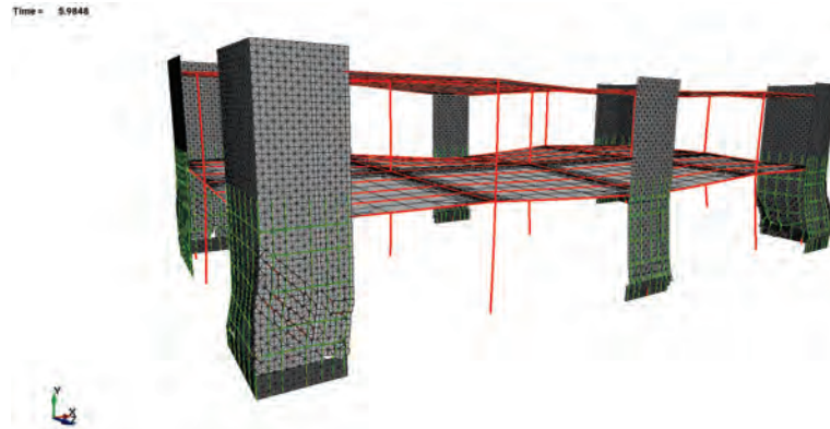
Figure B-45 Deformed meshes from refined model: COM5 (LS-DYNA) – Motion 1 ( MCE_R ).
